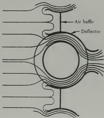
FIGURE 6-43. Cylinder baffle and deflector system.
